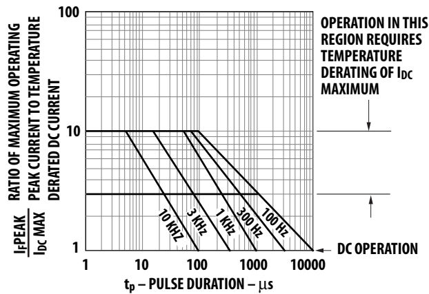
Figure 4. Maximum tolerable peak current vs. pulse duration – HER.
