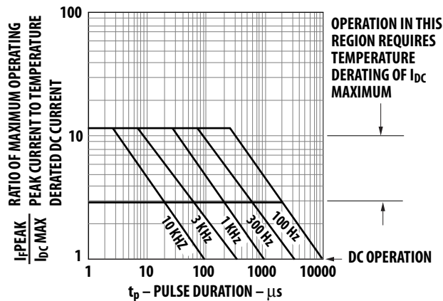
Figure 6. Allowable peak current vs. pulse duration – Green.
