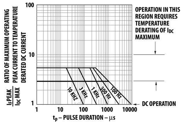
Figure 5. Maximum tolerable peak current vs. pulse duration – Yellow.
