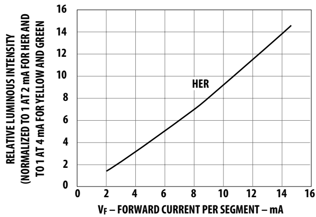
Figure 12. Relative luminous intensity vs. DC forward current.
