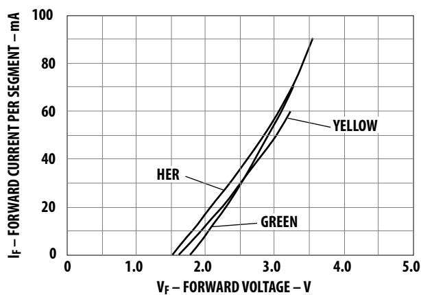
Figure 8. Forward current vs. forward voltage characteristics.
