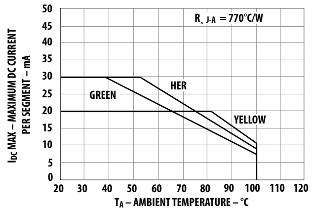
Figure 7. Maximum allowable DC current per segment as a function of ambient temperature.
