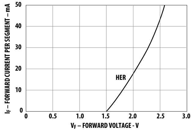
Figure 11. Forward current vs. forward voltage.
