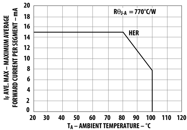
Figure 10. Maximum allowable average or DC current vs. ambient temperature.
